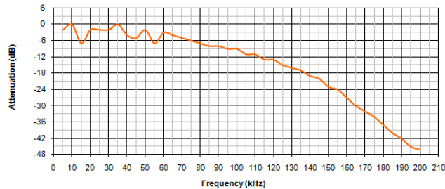
On-axis frequency response
